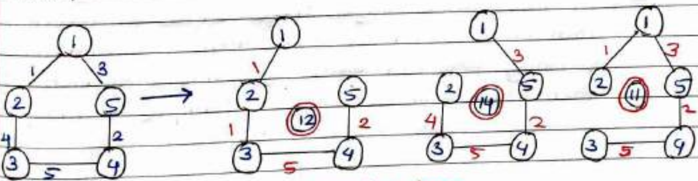
Graph
